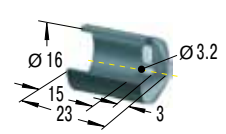
Steel Shroud
