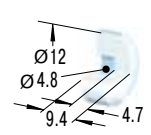
Nylon Button W 3 max = 14 Nm
