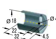
Steel Shroud
