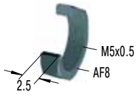
Locknut
