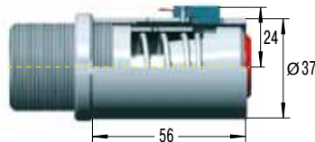
Switch Stop Collar
