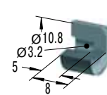
Steel Button
