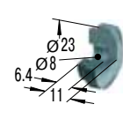
Steel Button
