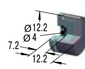
Steel/Urethane Button
