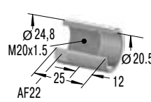
Stop Collar
