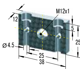
Universal Mount
