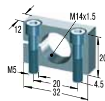
Clamp Mount
