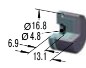
Steel/Urethane Button
