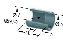
Stop Collar
